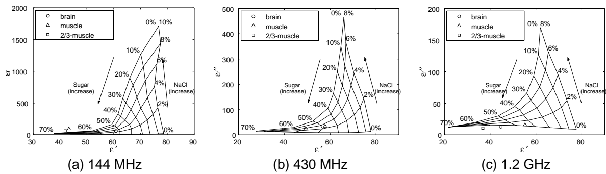
Figure 2: Complex permittivity of tissue-equivalent liquid.
