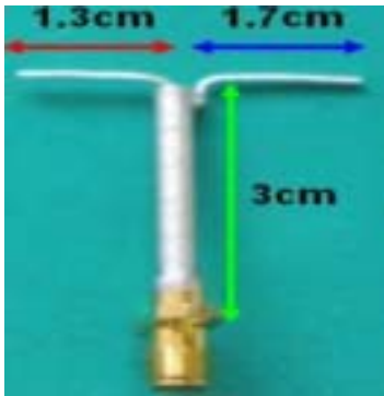
Fig. 1 The size of dipole antenna
