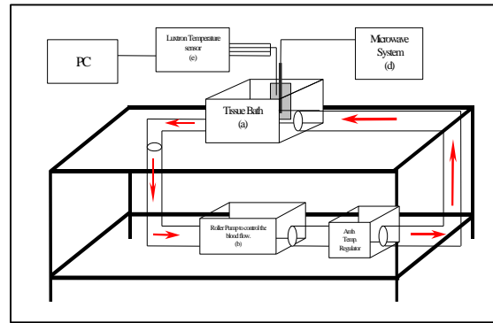
Figure 4. Equipment set up for the experimnt on a custom made trolley. The equipments are: (a) Tissue bath, (b) Roller pump, (c) Ambient Temperature Regulator, (d) Microwave system and (e) Luxtron optical fiber temperature sensor.
