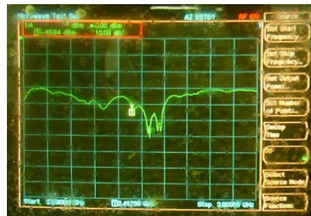
Figure 3: Measured results of 6 turns of the radial EBG structure.
