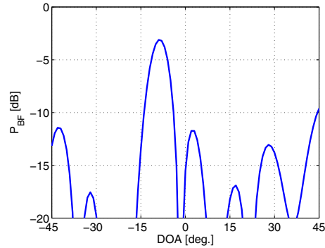
Figure 5: Estimated angular spectrum with the KR product expansion array processing (Doppler frequency shift at -0.500 [Hz])
