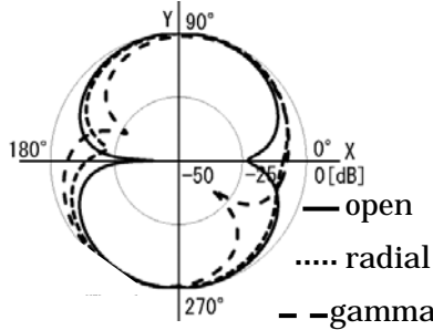
Fig.8. Radiation patterns of stubs in the XY plane for large transmission.
