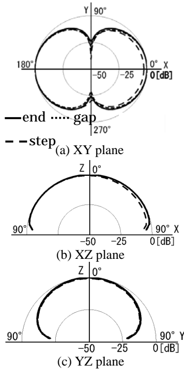
Fig.4. Radiation patterns of end, gap, and step.
