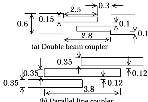
Fig.10. Couplers(in mm).
