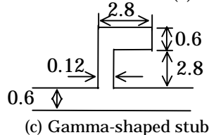
Fig.5. Stubs(in mm).
