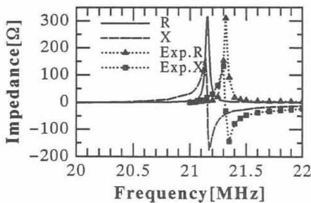
Fig.3 Input impedance of slotted tube resonator as a function of frequency for a/R_a=2.19
