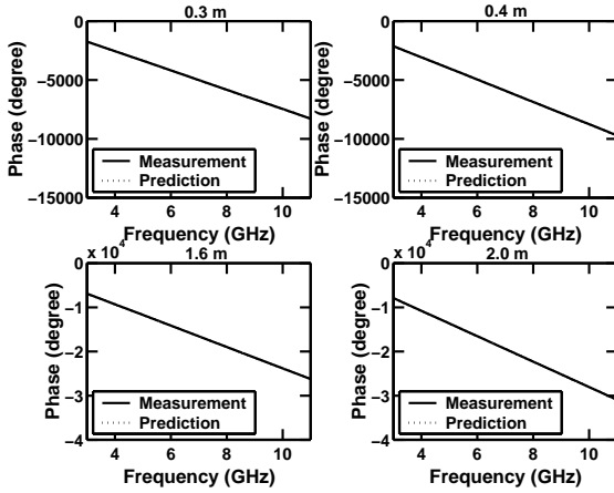
Figure 5: The phase of the transfer function of the UWB channel at 0.3, 0.4, 1.6 and 2.0 m distances.
