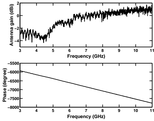
Figure 3: Magnitude (antenna gain) and phase of transfer function of each antenna.
