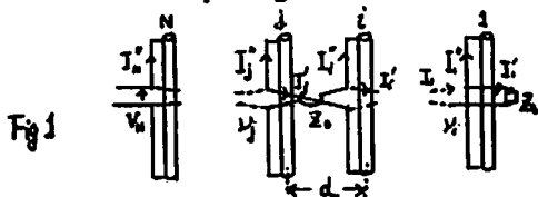
Analyzing method of transposed folded dipole array [2]
