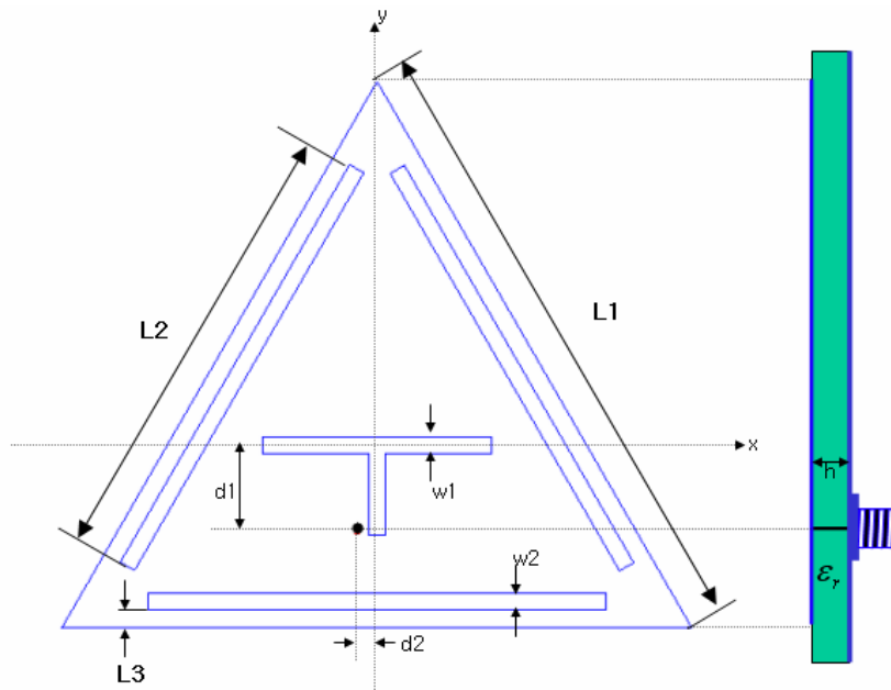
Fig. 1. Geometry of the proposed antenna.
