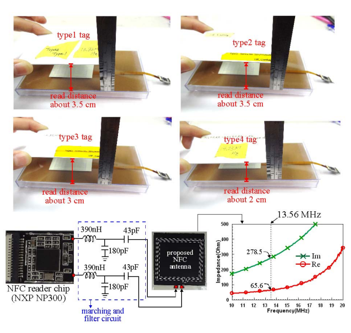
Fig. 3. Experimental photos and measured results for the proposed compact multi-layer NFC antenna by LITA process.
