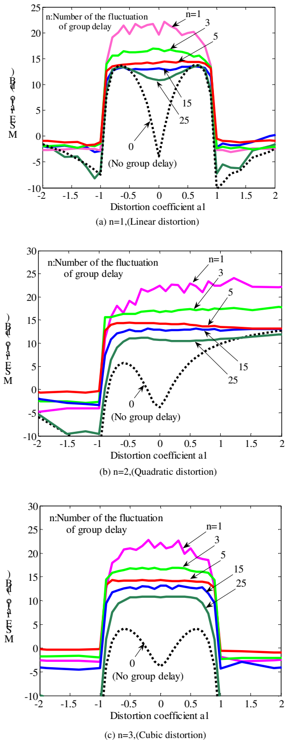
Fig.4 Influence of gain distortion on compensation effect
