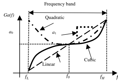
Fig.3 Gain characteristics of antenna
