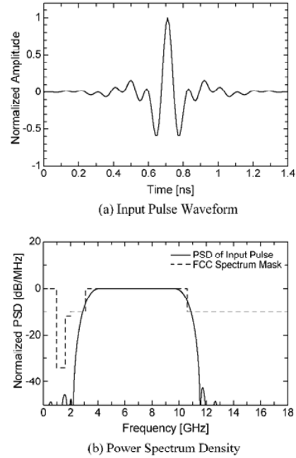
Fig. 8: (a) Time-domain waveform and (b) power spectrum density of the source pulse. The source pulse is a modulated cosine roll-off pulse with parameters f_c = 6.85 GHz, B = 7.5 GHz, and \alpha = 0.25 .
