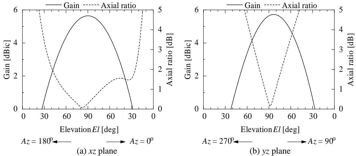
Fig. 2 Antenna performances in the azimuth plane
