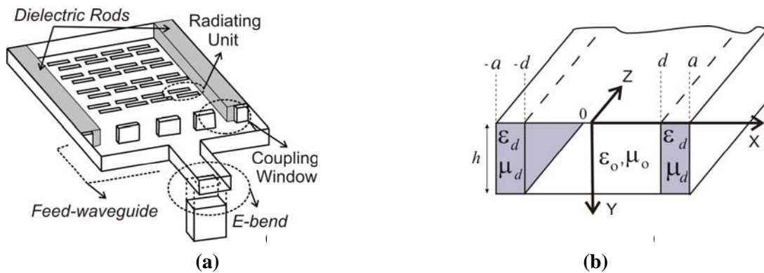
Figure 1: (a) Antenna outline, (b) Analysis model of a partially dielectric filled rectangular waveguide.
