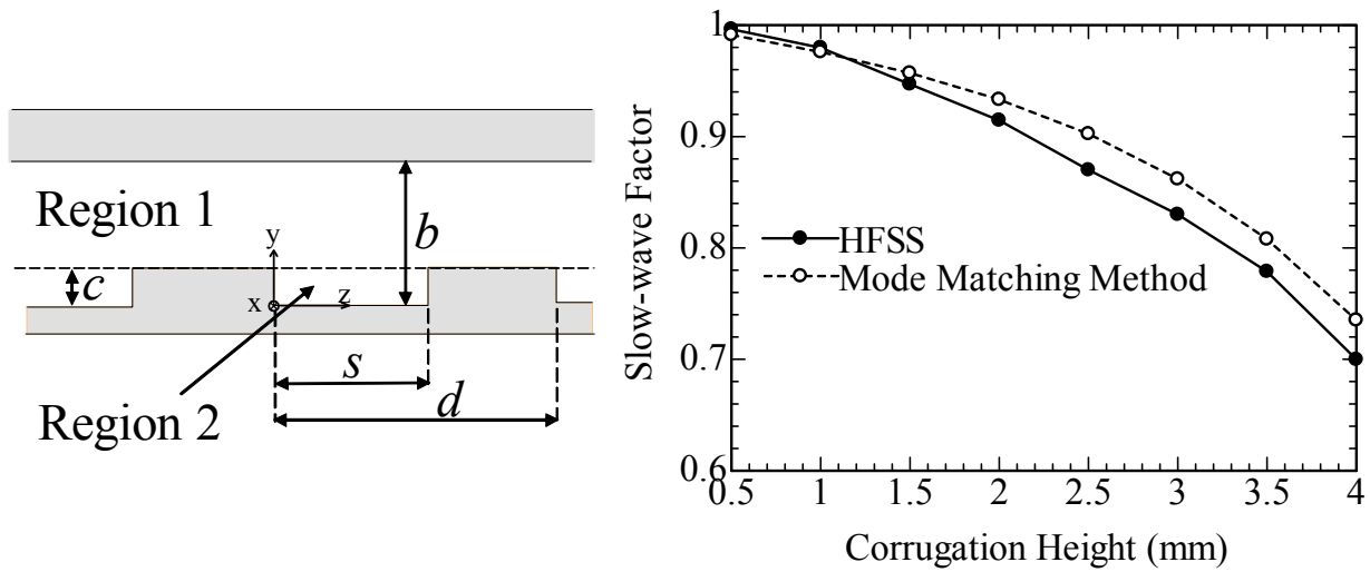
Figure 3: Analysis model for the mode matching method
