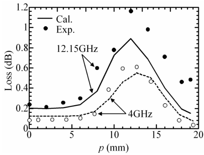
Fig.7 Loss as a function of the dielectric position p
