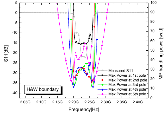
Fig. 3: Simulated MP free RF handling input power between each resonator end and wall surface with operating frequencies
