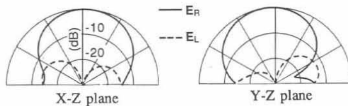
Fig.4 Radiation patterns
