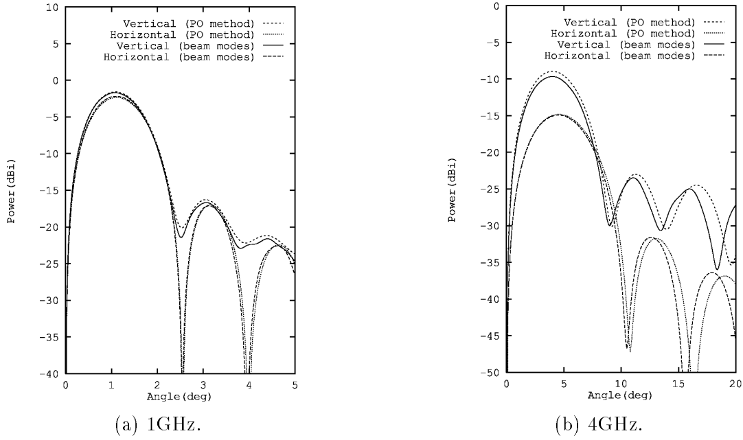
Figure 3: Comparisons between radiation patterns of cross-polar field in planes of symmetry ( \varphi_2 = 0^\circ ) and asymmetry ( \varphi_2 = 90^\circ ) calculated by the PO method and the presented beam modes analysis, where the distance r is infinity.
