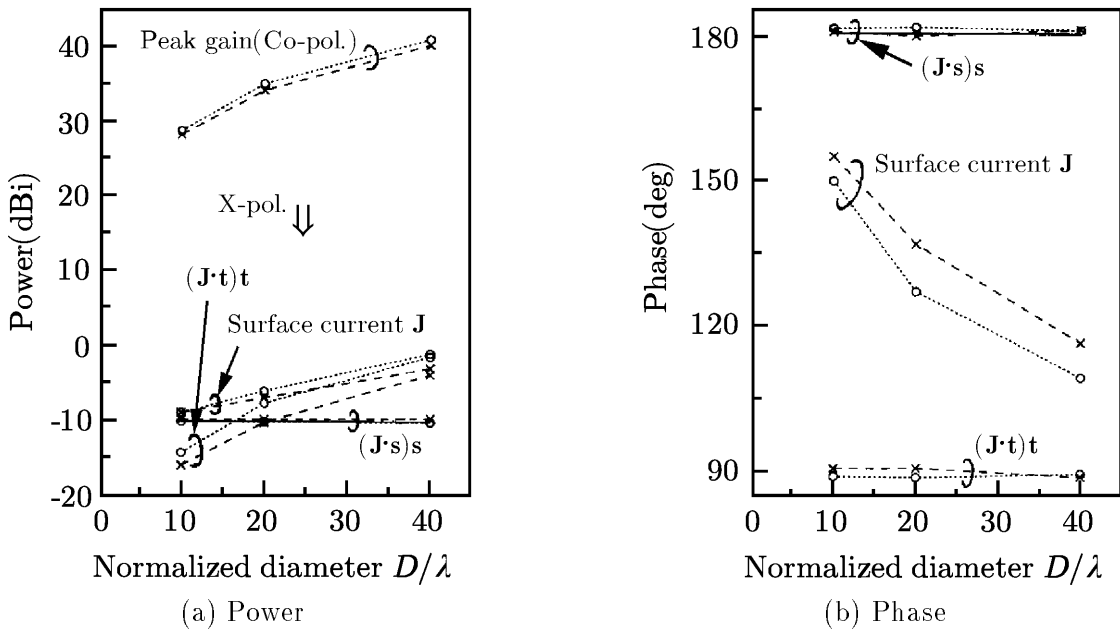
Figure 4: Peak value of the cross-polar field for vertically polarized excitations, where \mathbf{s}(= \mathbf{u}_{z2}) is the unit vector along the ray reflected by the reflector and \mathbf{t} is the unit vector along the normal current to the vector \mathbf{s} .
