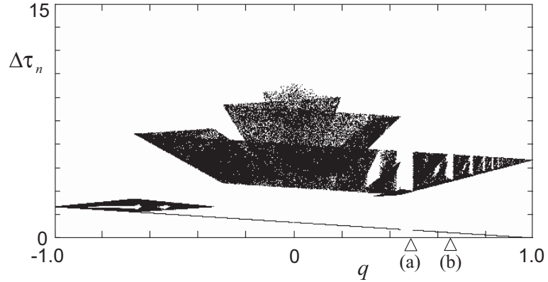
Figure 6: Bifurcation phenomena for a = 5 .
