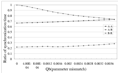
Figure 8: Relationship of the ratio of the synchronization time and small parameter mismatches. p = 2 , q = 3 , Q_a = 0.050 , a_1 = 1.70 , a_2 = 1.98 and \varepsilon = 0.40 . The number of iteration is 1000000.
