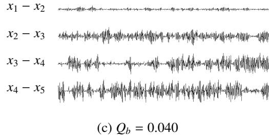
Figure 7: Variable differences between two subsystems. p = 2 , q = 3 , Q_a = 0.050 , a_1 = 1.70 , a_2 = 1.98 and \varepsilon = 0.40 .
