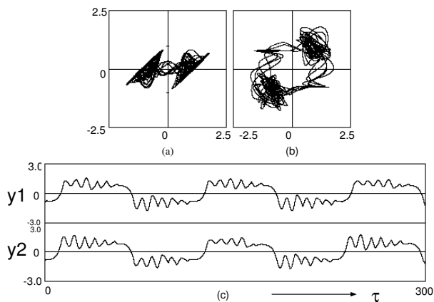
Figure 3: State transition phenomenon around in-phase synchronization (computer calculated result). \alpha = 1.5 , \beta = 5.0 , \gamma = 0.2 , and \delta = 0.008 . (a) Attractor on y_1 - z_1 plane. (b) Attractor on y_1 - y_2 plane. (c) Time waveform.
