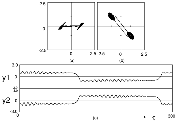
Figure 5: State transition phenomenon around anti-phase synchronization (computer calculated result). \alpha = 2.0 , \beta = 4.0 , \gamma = 0.1 , and \delta = 0.0014 . (a) Attractor on y_1 - z_1 plane. (b) Attractor on y_1 - y_2 plane. (c) Time waveform.
