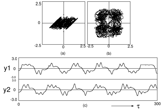
Figure 7: Computer calculated result corresponding to Fig. 6. \alpha = 1.5 , \beta = 5.0 , \gamma = 0.2 , and \delta = 0.015 . (a) Attractor on y_1 - z_1 plane. (b) Attractor on y_1 - y_2 plane. (c) Time waveform.
