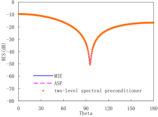
Figure 1. Bistatic RCS of the dielectric sphere
