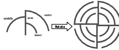
Figure 1. Gemetry of the proposed bionic FSS
