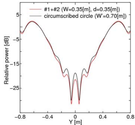
Figure 7: Comparison of the relative power for the equivalent cylinder. ( X_0 = 1.0\text{m} )
