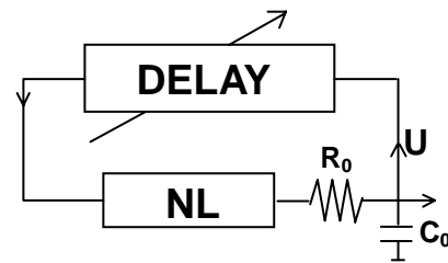
Fig.1 Block diagram of the Mackey-Glass electronic circuit
