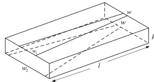
Figure 3. The microstrip line-parallel wire balancer
