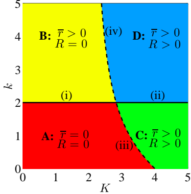
Figure 1: Phase space for Eq. (1) with \delta, \Delta = 1 . Regions A, B, C, and D (described in the text) are denoted in red, yellow, green, and blue, respectively, with bifurcations (i)–(iv) indicated by solid and dashed curves.
