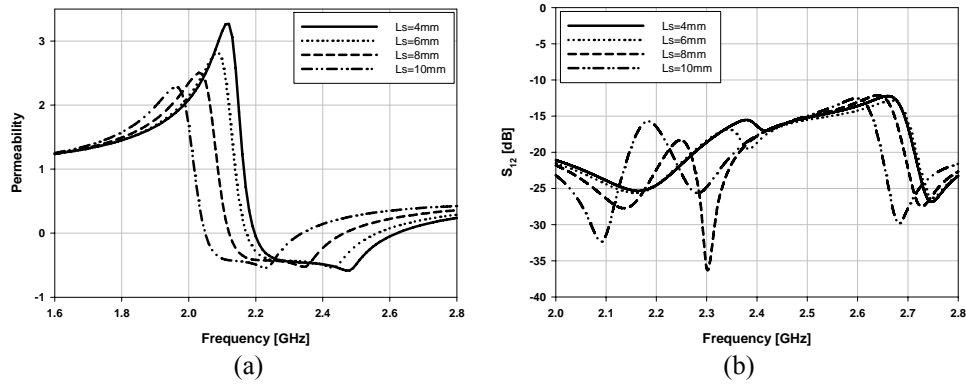
Figure 3: Simulated effective permeability and S_{12} characteristics : (a) Effective permeability for variation in L_s , (b) isolation for variation in L_s .
