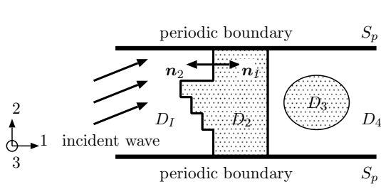
Fig. 1: Periodic boundary value problems
