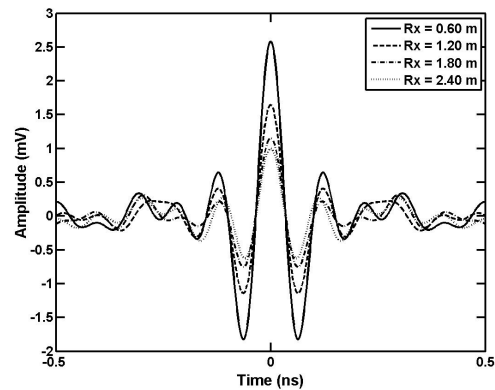
Figure 4: Received signal output of the matched filter: optimum.
