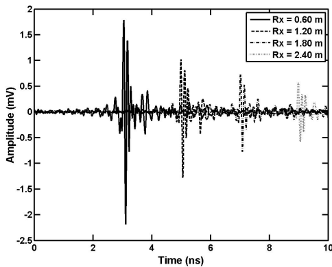
Figure 3: Received signal waveform at the antenna output.
