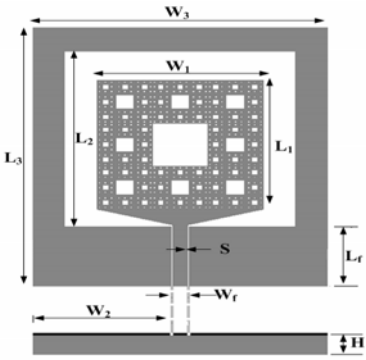
Figure 2: The configuration of the proposed antenna 2
