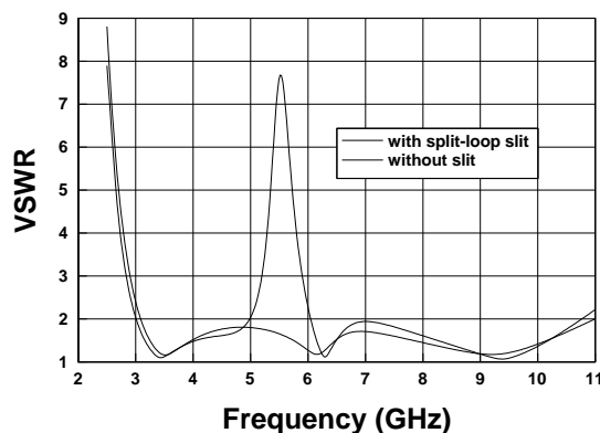
Fig. 2 Simulated VSWR for the band-notch UWB antenna with split- loop slit and without slit
