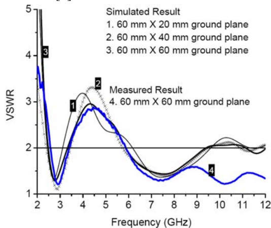
Figure 5: Simulated and Measured VSWR
