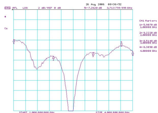
Figure 21: Return Loss
