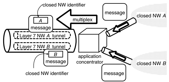
Fig. 1: Multiplexing the content of communications at the application layer
