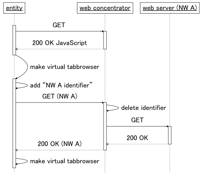
Fig. 9: Communications using Web concentrator
