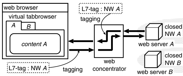
Fig. 7: Web concentrator
