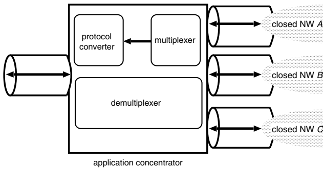
Fig. 3: Overview of application concentrator
