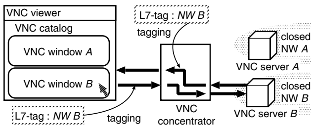
Fig. 11: VNC Concentrator
