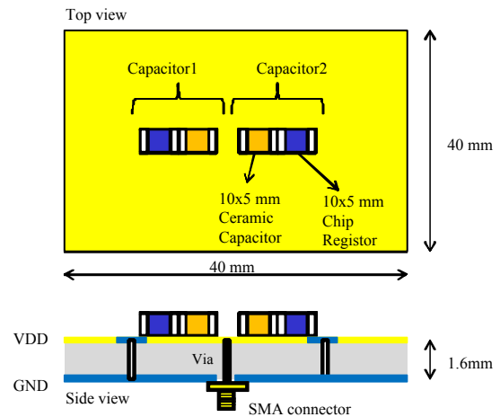
Fig. 6. Test board and instrumental setup for experiments.
