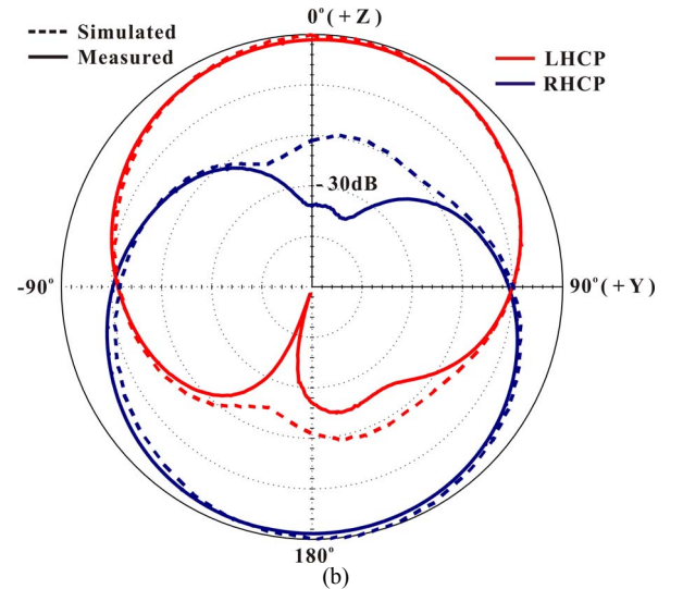
Figure 3. Simulated and measured normalized LHCP / RHCP radiation patterns for the proposed broadband CP antenna at 940 MHz. (a) X-Z plane. (b) Y-Z plane.
