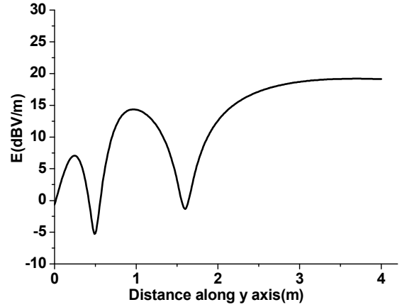
Figure 8. Electric field intensity of measuring points along y axis, while h=0
