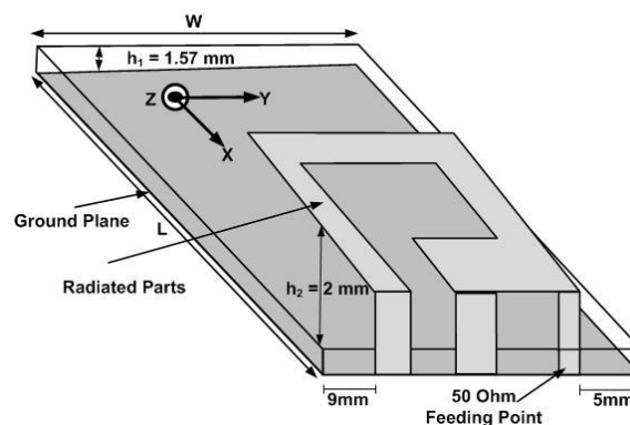
Fig. 1 The layout of the proposed antenna
