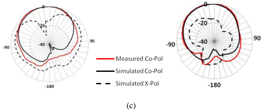
Fig. 3 The Simulated and measured E and H planes Co and X-pol radiation patterns for the proposed antenna (a) The orientation of the antenna (b) 2.09 GHz (c) 3.74 GHz and (d) 5 GHz.
