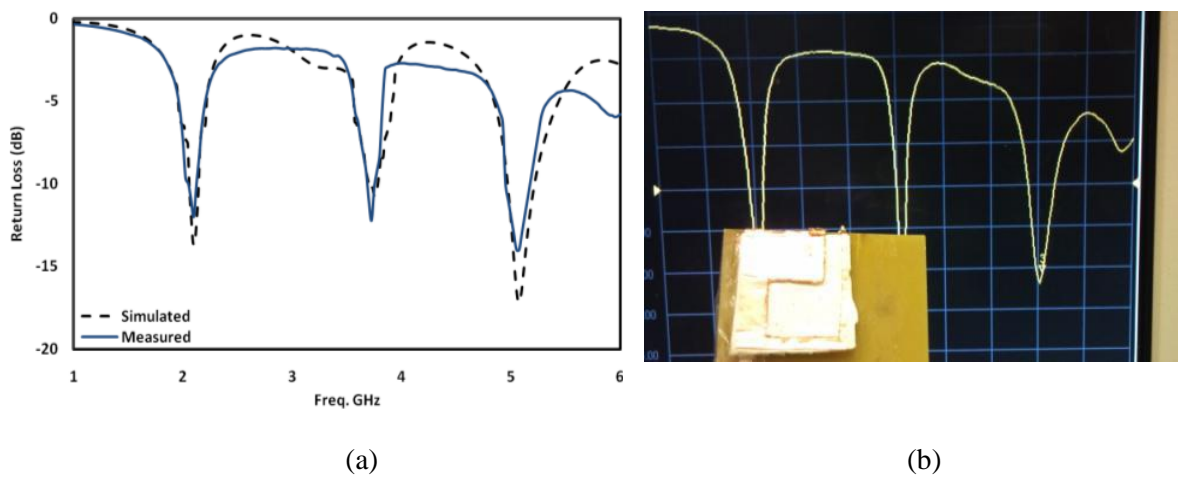
Fig. 2 (a) The simulated and measured return loss S_{11} (b) The fabricated prototype of the proposed antenna connected to the network analyser.
