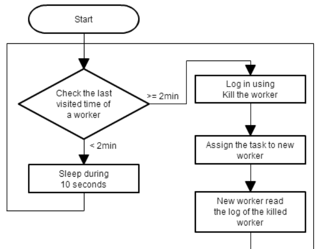
Fig. 5. Recovery of a crawling task
