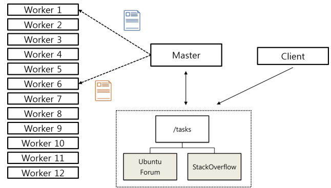
Fig. 3. Distributing crawling tasks to workers
