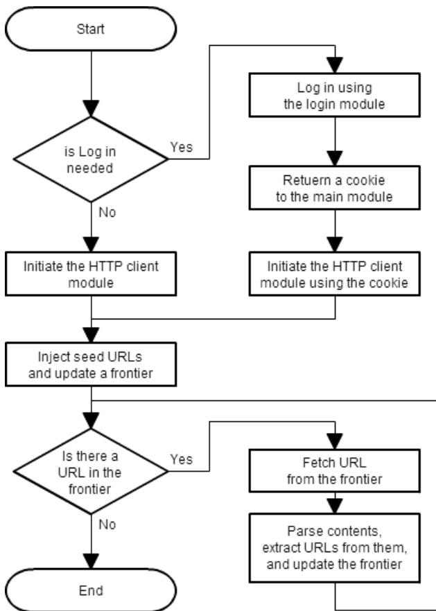
Fig. 4. How the main module works
