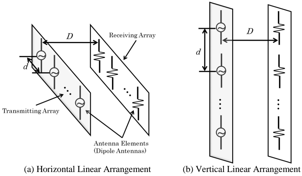
Figure 2: Analysis Models of Near-field MIMO System
