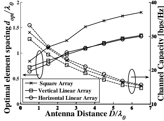
Figure 3: Optimal Element Spacing at Certain Antenna Distance
