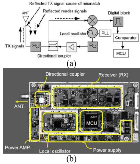
Fig 5. Entire reader block diagram (b) pictured prototype
