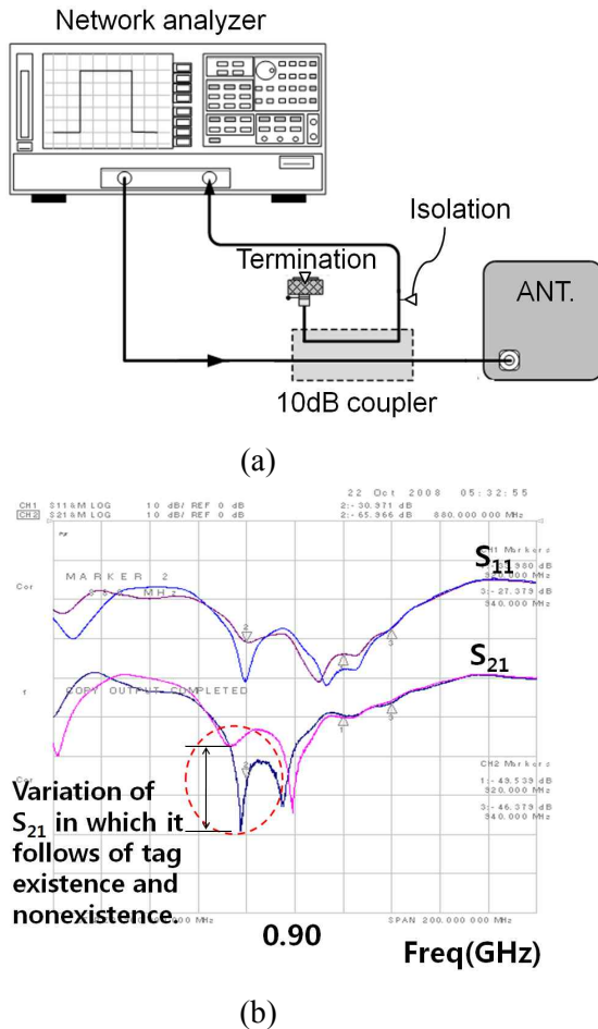
Fig 4. (a) Measurement composition using network analyzer (b) measurement results respecting two cases (with/without chipless tag)
