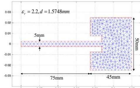
Fig.1. Planform of a patch antenna meshed by triangles
