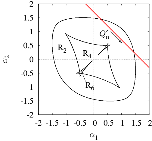
Figure 2: Numerical result on existence and number of equilibrium points. In the region R_2 (or R_4 , R_6 ), there are two (or four, six) distinct equilibrium points of the dynamical model (6).
