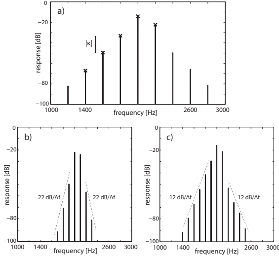
Figure 1: CT in a single Hopf oscillator. a) Fourier transform of the response of a single Hopf oscillator ( \omega_{ch} = 2\pi \cdot 2000 rad/s, \mu = 0 ) when subject to two-tone forcing ( \omega_1 = 2\pi \cdot 2000 rad/s and \omega_2 = 2\pi \cdot 2200 rad/s with amplitudes F_1 = F_2 = 0.01 ); spectrum: numerical integration, crosses: analytical results; exponential decay factor |\kappa| = \left| \frac{\omega_{ch} a_1 a_2^*}{i\omega_0} \right| from Eq. (11). b), c) Same experiment as in a), with \omega_{ch} = 2\pi \cdot 1900 rad/s, \omega_{1,2} = 2\pi \cdot (2000, 2100) rad/s and amplitudes F_1 = F_2 = 0.01 , where b) \mu = -0.1 and c) \mu = 0 (oscillator at criticality).
