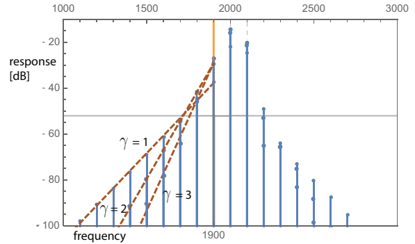
Figure 3: CT decay, generalized Hopf cochlea, \gamma = 1, 2, 3 .
