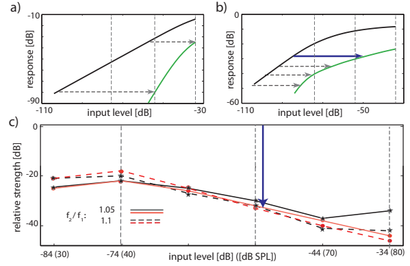
Figure 2: The behavior of the first cubic CT in a single Hopf element, in the compound cochlea and in biology. a), b) Response amplitude to a pure tone of frequency f_{ch} (black), response to a two-tone input (equal strength of components) with f_{ch} = f_{CT1} (green). The difference (arrows) is the ‘relative strength of CT1’. a) Single Hopf amplifier (no fluid comprised), and b) cochlea section 6 where f_{ch} = f_{CT1} . c) Relative strength of CT1 for two f_2/f_1 -frequency ratios. Red: cochlea section 6, black: biological data [6] ( f_{ch} = 9000 Hz). The blue arrows in b) and c) describe the same experimental result.
