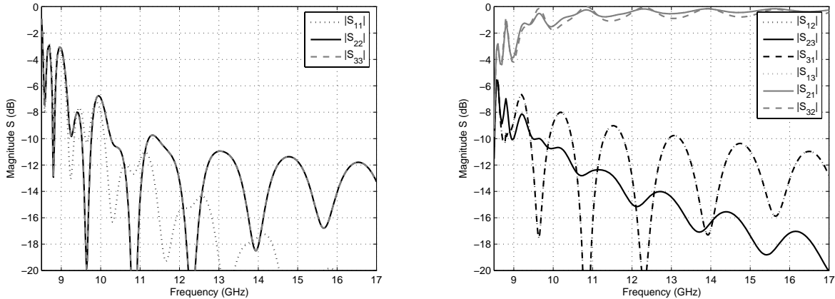
Figure 3: Predicted scattering matrix of the ferrite coupled line circulator: a) reflection losses, b) insertion losses and isolations
