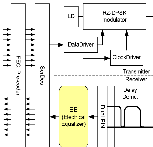
Fig.1 Transponder configuration
