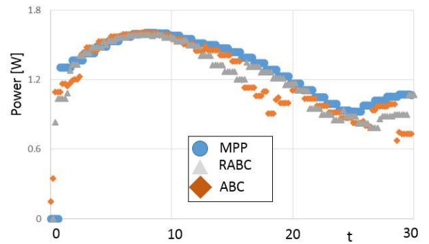
Figure 6: MPPT process.
