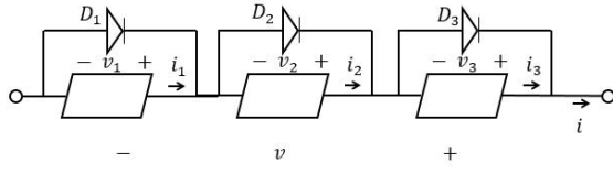
Figure 1: Photovoltaic System
