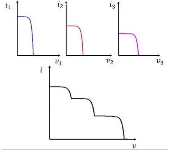
Figure 3: Voltage-current characteristics
